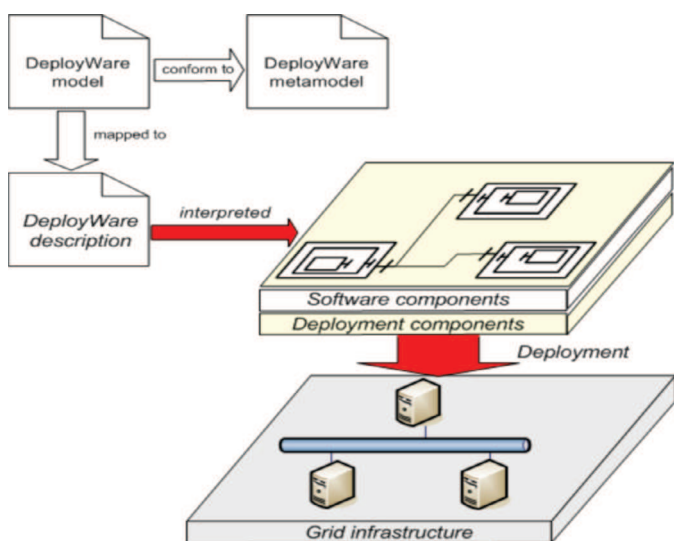
Fig. 18. DeployWare architecture (Flissi et al., 2008).
