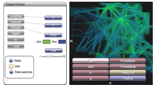
Figure 2: FromDaDy overview.
