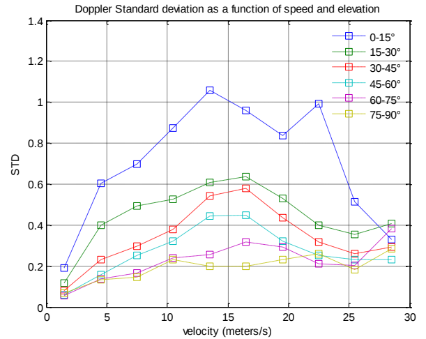
Figure 20 Estimated standard deviation of Doppler multipath on uBlox receiver + patch antenna, as a function of speed and elevation
