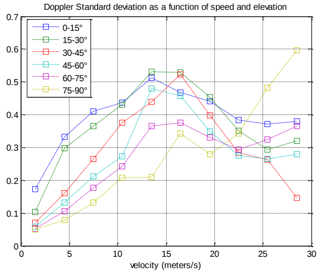
Figure 11 Estimated standard deviation of Doppler multipath on uBlox receiver (4Hz data), as a function of speed and elevation. Standard deviation was estimated for speed “slices” of 3\text{m.s}^{-1} , from 0 to 30\text{m.s}^{-1}
