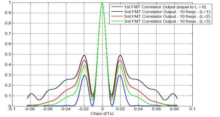
Figure 12: Normalized non-coherent correlator C output
