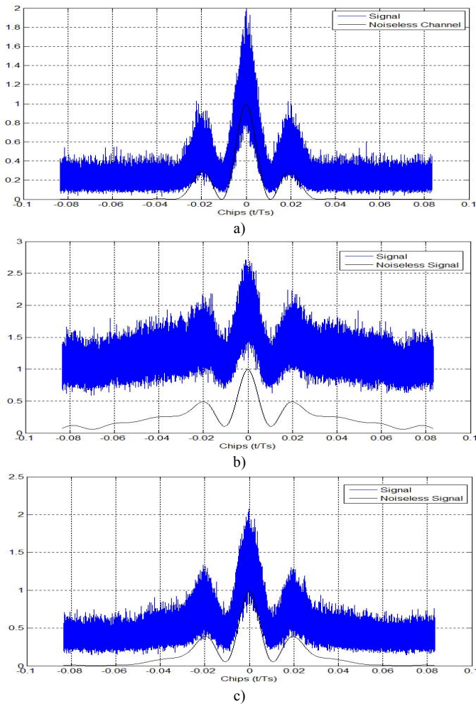
Figure 16: Normalized correlator output vs signal code delay estimation error. C/N_0 = 15 dB-Hz and non\_coh = 24PRN . a) Correlator A ( coh = 1PRN ). b) Correlator B ( L = 1, coh = 1PRN ). c) Correlator C ( L = 3, coh = 3PRN ).
