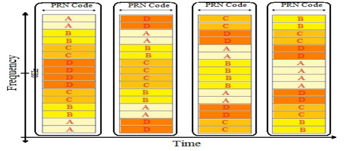
Figure 14: Coherent and non-coherent operations of the acquisition process of the 3 rd data distributions for the 1 st option correlator
