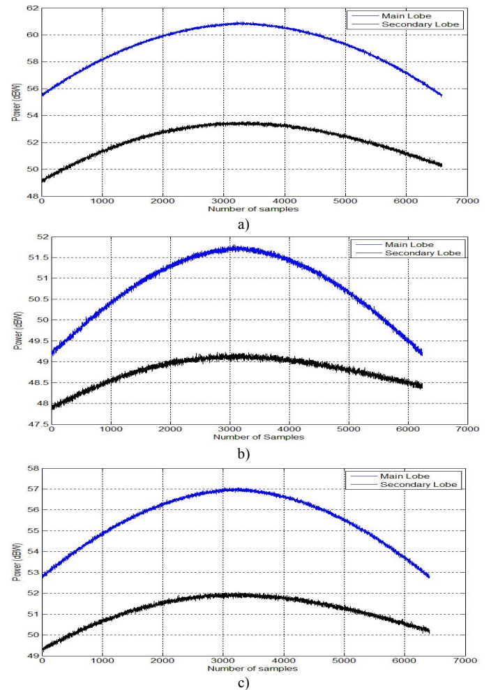
Figure 17: Correlator output main lobe and secondary lobe average power. C/N_0 = 15 dB-Hz and non\_coh = 24PRN . a) Correlator A ( coh = 1PRN ). b) Correlator B ( L = 1, coh = 1PRN ). c) Correlator C ( L = 3, coh = 3PRN ).
