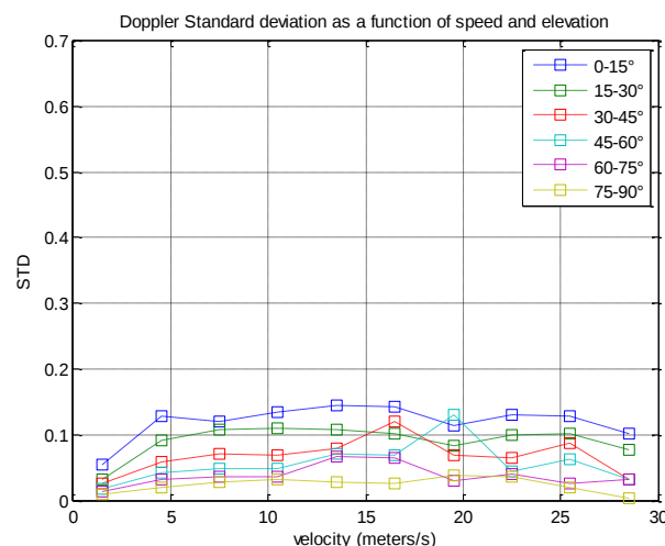
Figure 10 Estimated standard deviation of Doppler multipath on Novatel receiver (1Hz data), as a function of speed and elevation. Standard deviation was estimated for speed “slices” of 3\text{m.s}^{-1} , from 0 to 30\text{m.s}^{-1}
