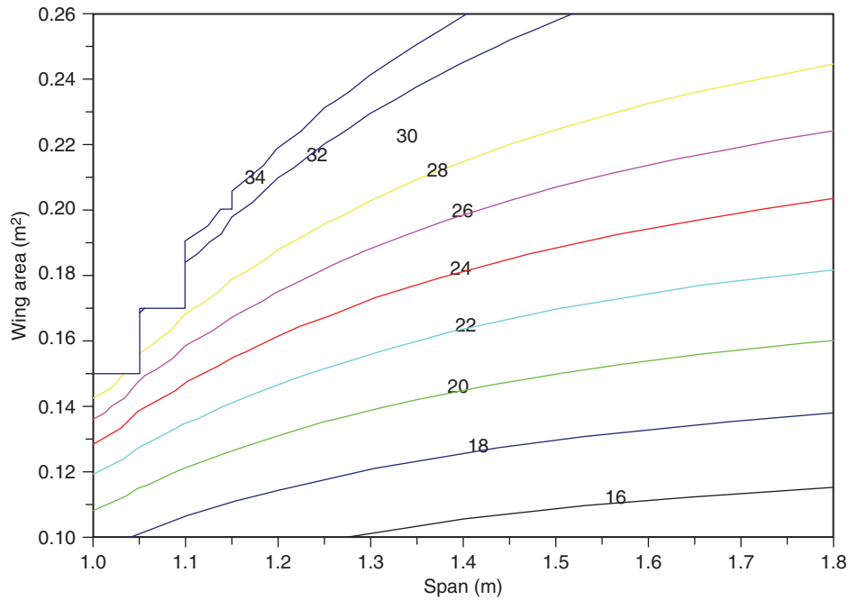
Figure 7. Total weight ( N ) at 20\text{ m/s} cruise speed for a 200\text{ km} mission.
