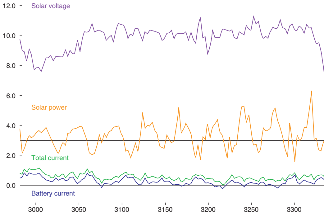
Figure 15. Solar Voltage ( Volt ), Solar Power ( W ), Total (solar+battery) and Battery Current ( A ) during 300s of flight. When the battery current is non positive, the battery is charged.
