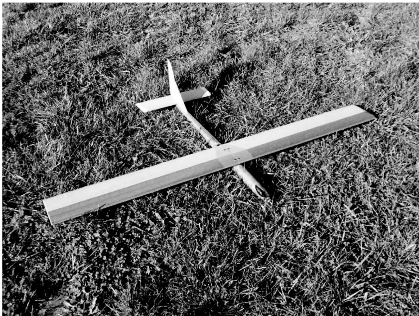
Figure 9. The 200 km mission prototype ready for its first flight.
