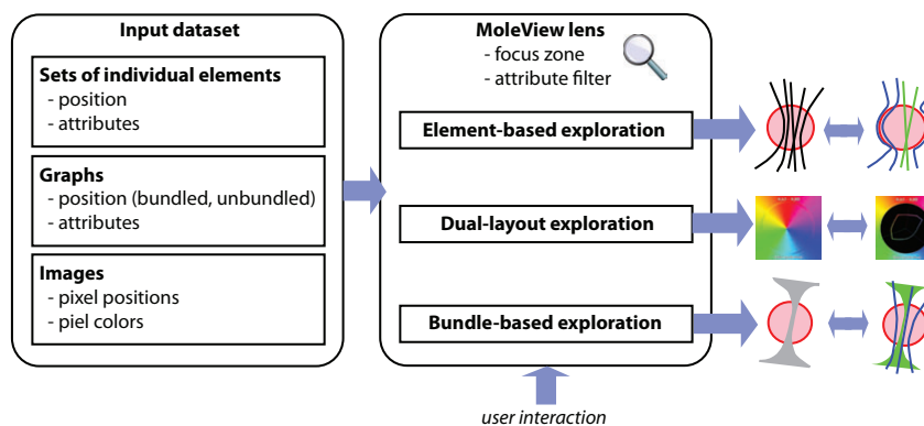
Figure 1: MoleView interactive exploration pipeline
