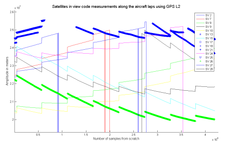
Figure 8: GPS L2 code measurements during recording for all satellites in view
