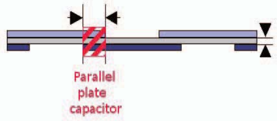
Figure 5: Parallel plate capacitor realised on each side of 25 \mu\text{m} of Kapton.
