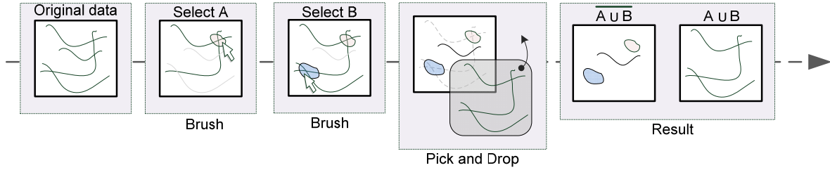
Fig. 7. Union Boolean operation
