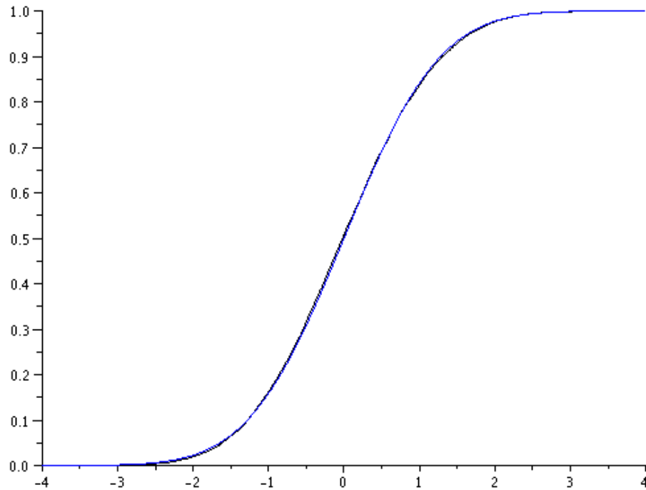
Figure 5. Comparison of measured Cumulative Distribution Function (black) and computed normal law CDF (blue)
