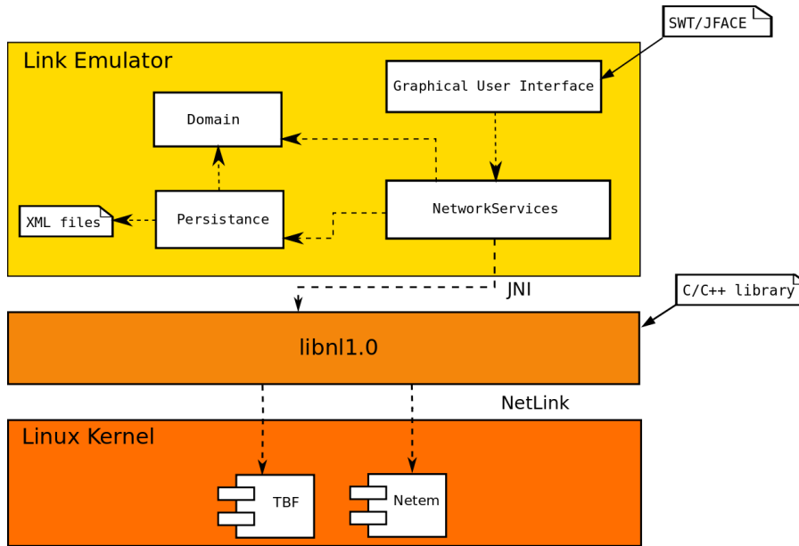
Figure 3. Software Architecture of the link emulator
