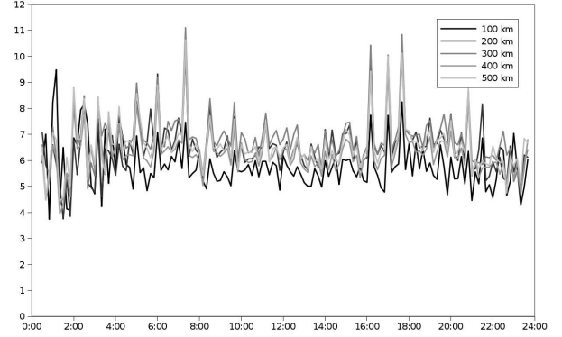
Figure 10. standard deviation of the signal-to-noise ratio of all useful signals during a day for different ranges
