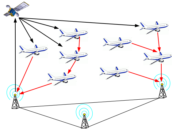
Figure 13. Hybrid topology
