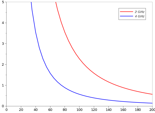
Figure 6. Throughput (Mbps) evolution with the distance (km)
