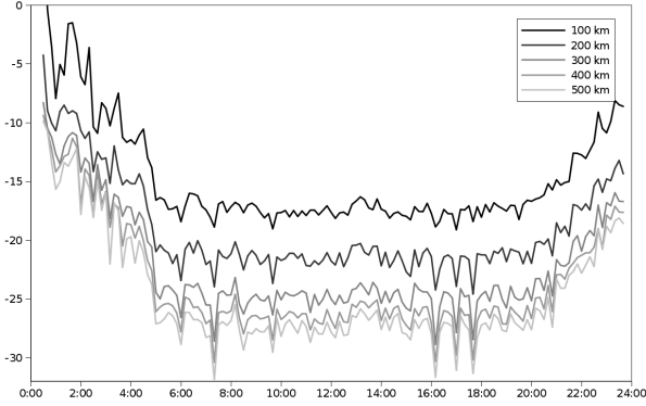
Figure 9. Average of the signal-to-noise ratio (dB) of all useful signals during a day for different ranges
