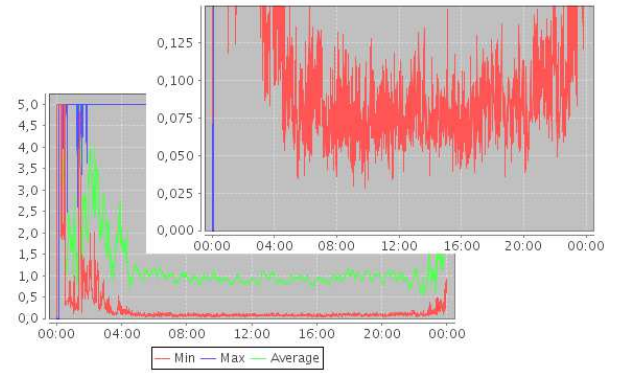
Figure 8. Fairly shared available throughput (Mbps) per aircraft
