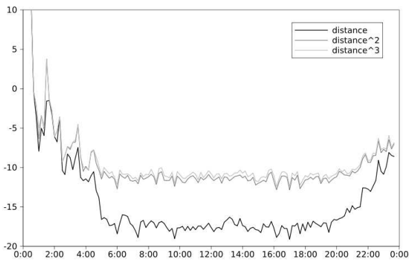
Figure 12. Average of the signal-to-noise ratio (dB) of all useful signals during a day for different edges weights
