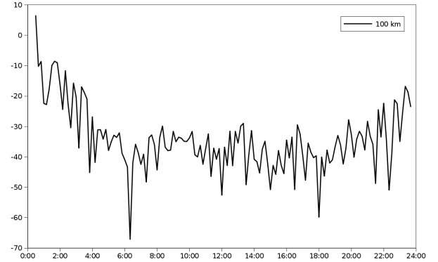
Figure 11. Minimum of the signal-to-noise ratio of all useful signals during a day for a range of 100 km
