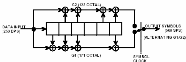
Fig. 10: Convolutional Encoding
