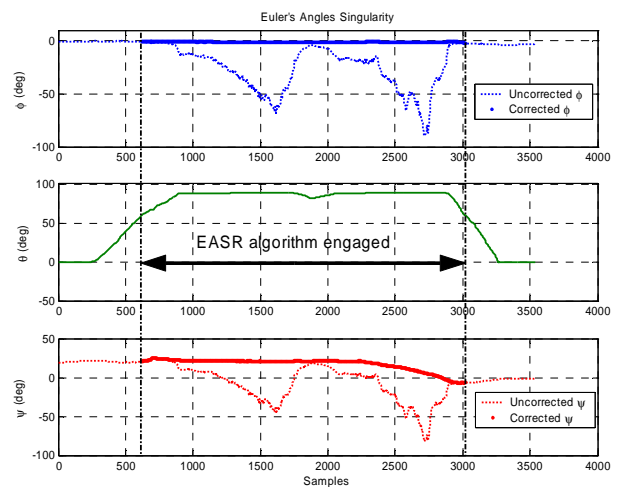
Figure 9 – Euler's angles singularity resolution.
