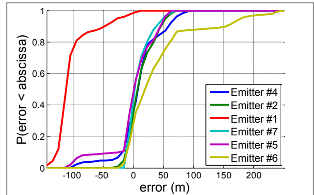
Fig 19 - CDF of error for each tracked emitter of the SFN
