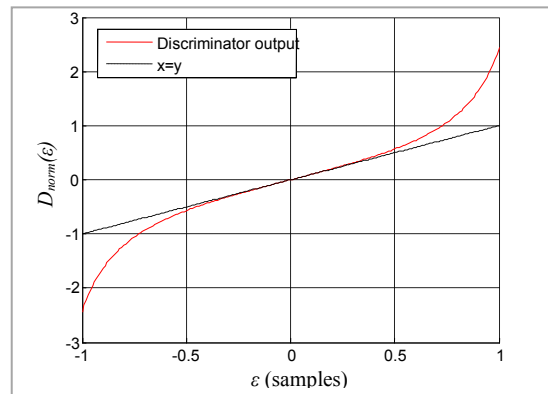
Fig 9 - Normalized |E|^2 - |L|^2 discriminator output
