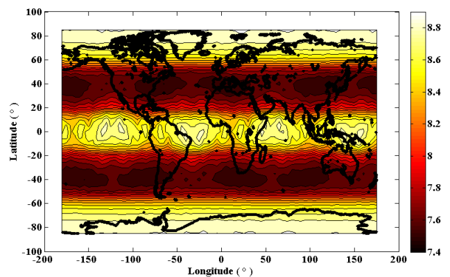
Figure 5 - Average number of satellites over 1 day considering 24 satellites GPS constellation
