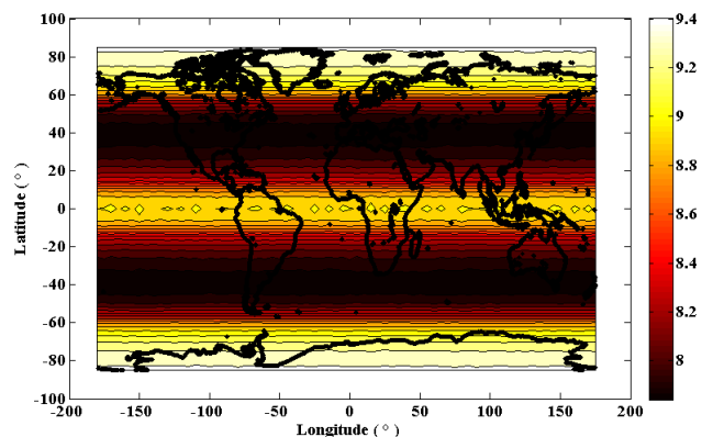
Figure 6 - Average number of satellites over 1 day considering 27 satellites Galileo constellation (mask angle 10^\circ )
