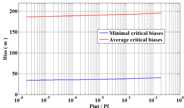
Figure 7 - Smallest bias that leads to a positioning failure - APVI operations (HAL=40m,VAL=50m) – dual constellation (GPS + Galileo)
