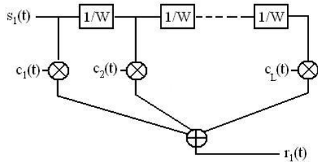
Figure 5: Mathematical model for a frequency-selective channel - A truncated tapped delay line
