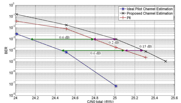
Figure 9: Comparison between ideal pilot channel estimation, proposed pilot channel estimation and PLL tracking method for GPS L1C: BER vs C/N0 (dBHz)
