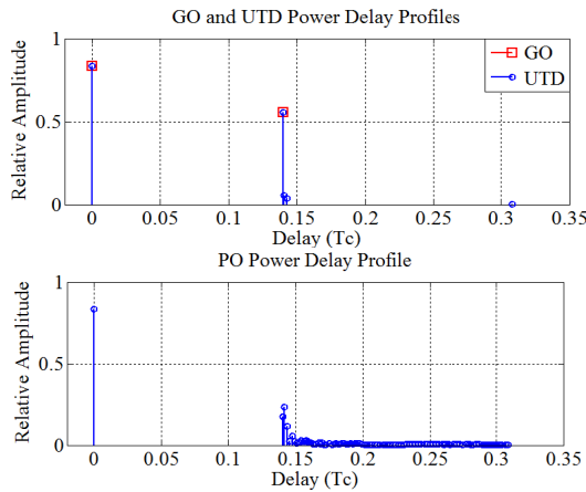
Fig. 5 Comparison of the GO, UTD and PO Power Delay Profiles
