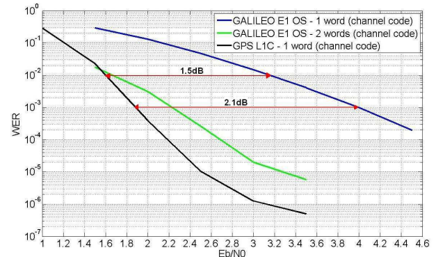
Figure 5: Comparison of the ephemeris decoding performance only depending on the implemented channel code between GPS L1C and GALILEO E1 OS: WER vs E_b/N_0 (dB)
