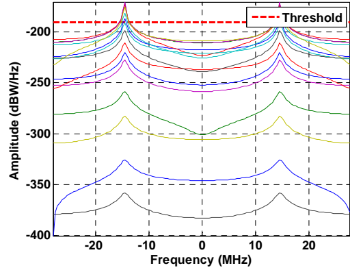
Figure 9 : Comparison of signal FFTs to FDAF threshold.
