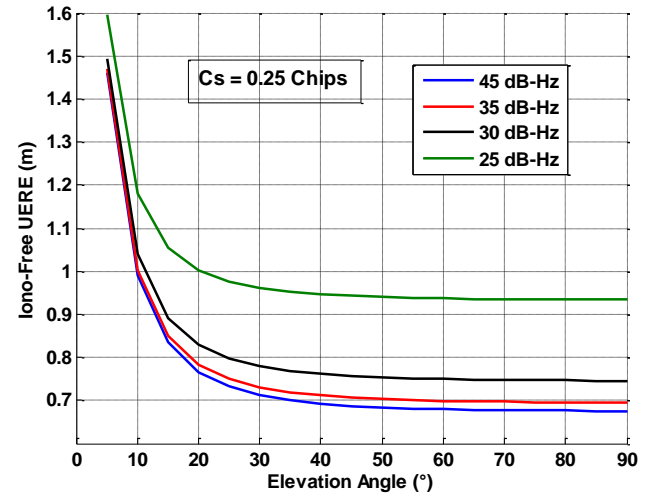
Fig 1 - Galileo smoothed iono-free UERE for C/N0=45 dB-Hz on E5b and different C/N0 on E1
