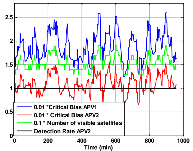
Fig 5 - Sequential Constrained GLR RAIM-APV 1 &2 Reference Simulations- Nominal Conditions
