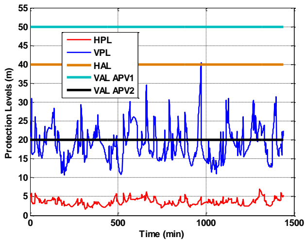
Fig 10 - RAIM LSR-APV 1 & 2 - Nominal Conditions
