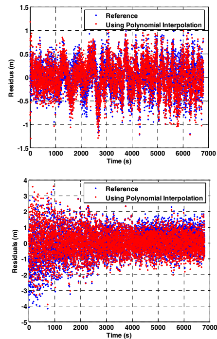
Figure 3 – Comparison of Pseudorange Residuals Obtained Through Polynomial Interpolation and CMC
