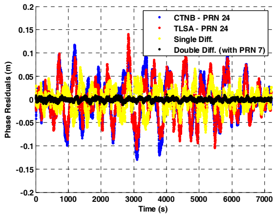
Figure 11 – Polynomial Interpolation Residuals for Raw, Single-Differenced and Double-Differenced Phase Measurements
