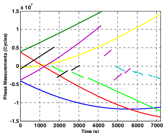
Figure 4 – Example of Carrier-Phase Measurements
