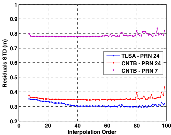
Figure 2 – Residual Standard Deviation Obtained Using Different Interpolation Order for Different Satellites and RIMS Stations
