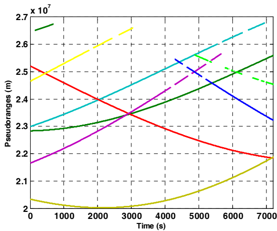
Figure 1 – Example of Pseudorange Measurements
