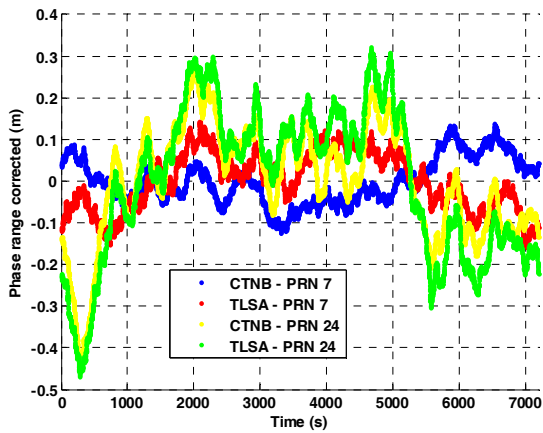
Figure 7 – Example of the Phase Measurement Refined Model Residuals
