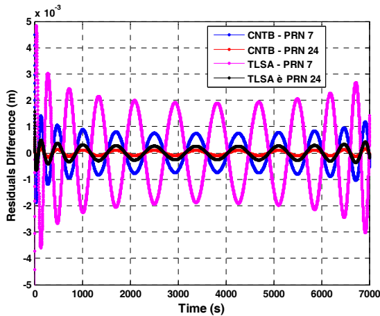
Figure 8 – Difference between Residuals Obtained from Polynomial Interpolation using Raw Phase Measurement and Refined Measurement Model
