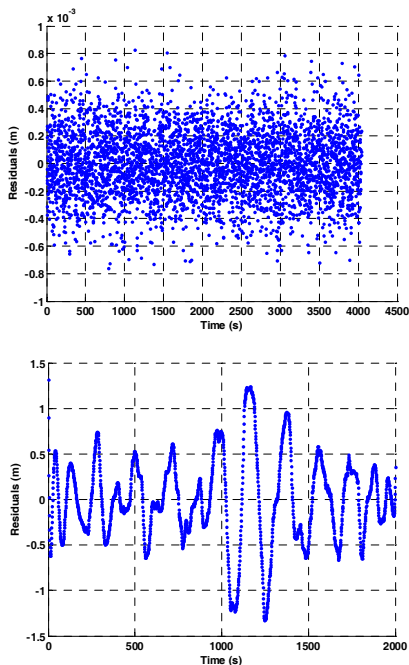
Figure 6 – Interpolation Residuals Obtained Using a Common Oscillator (Top) and Separate Ones (Bottom)
