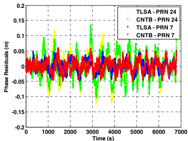
Figure 5 – Phase Residuals Obtained Through Polynomial Interpolation
