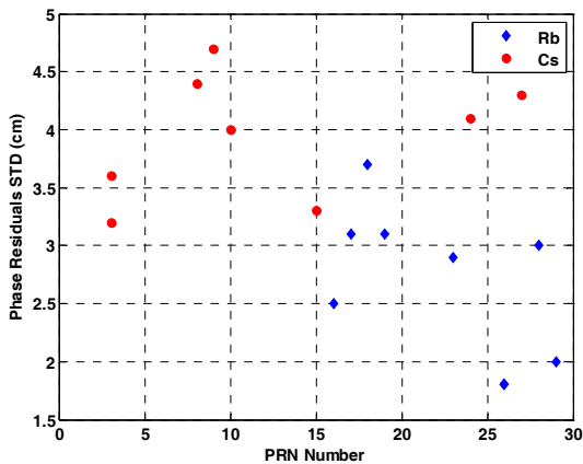
Figure 10 – Phase Residuals Standard Deviation Obtained from Polynomial Interpolation
