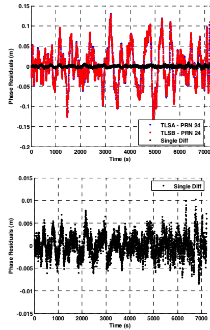
Figure 12 – Polynomial Interpolation of Raw Measurements and Single Differenced Phase Measurements Using RIMS Sharing a Common Oscillator (Zoom on the Bottom)
