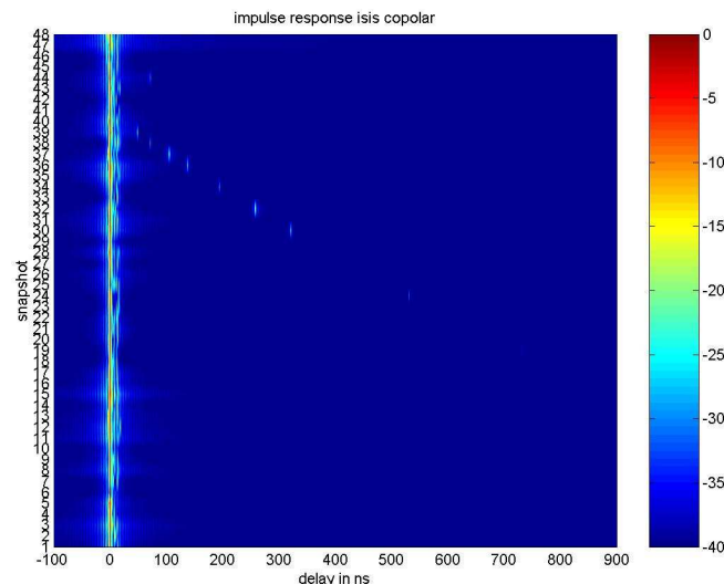
Figure 2: Channel impulse response of the final approach in a large time scale.
