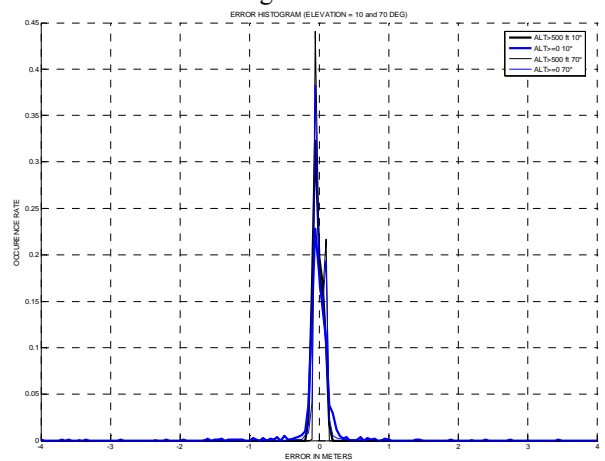
Figure 19: Unsmoothed code tracking error distribution at 10° and 70° (GPS L1 C/A, BW 2 =2 MHz, C S =1 chip, 500 approaches per sat elevation, A340).
