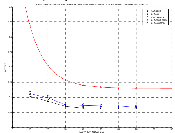
Figure 31: Smoothed pseudorange error sigma compared to SARPS model (GPS L1 C/A, BW_2=2 MHz,
