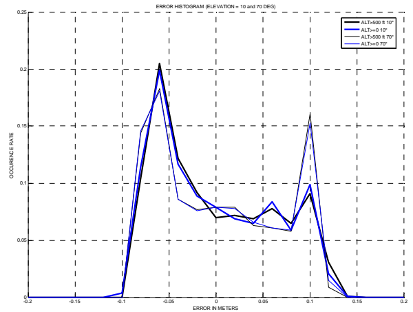
Figure 30: Smoothed pseudorange error distribution for sat elevation angles 10^\circ and 70^\circ (GALILEO BOC(1,1), BW_2=6 MHz, C_S=0.2 chip, 500 approaches per sat elevation, A340).
