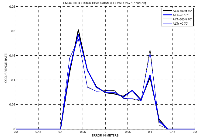
Figure 22: Observed distribution of smoothed code tracking errors for elevations 10° and 70° (GPS L1 C/A, BW2=16 MHz, C_S = 0.1 chip, no ground reflection, 500 approaches per sat elevation, A340).
