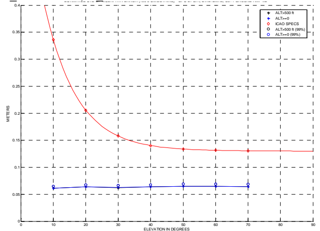
Figure 23: Smoothed pseudorange error sigma compared to SARPS model (GPS L1 C/A, BW2=16 MHz, C_S = 0.1 chip, 500 trials per elevation, A340).
