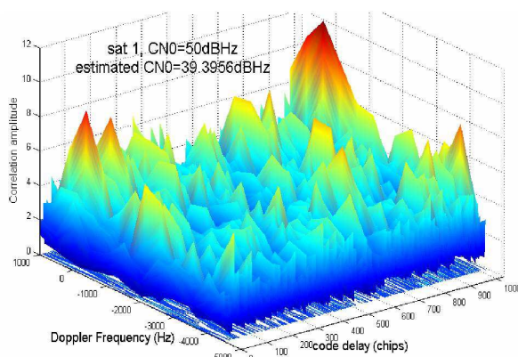
Fig 6: LOS signal of satellite 1 correlated with C/A code of satellite 11 to view the resulting cross-correlation function.
