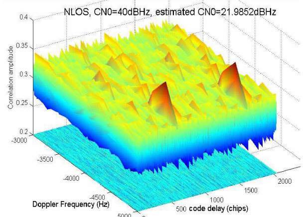
Fig 4: Non-LOS signal, multipath replicas only; initial C/N_0 40dBHz ( C/N_0 that affected the LOS that could not reach the receiver); estimated C/N_0 21.9852dBHz
