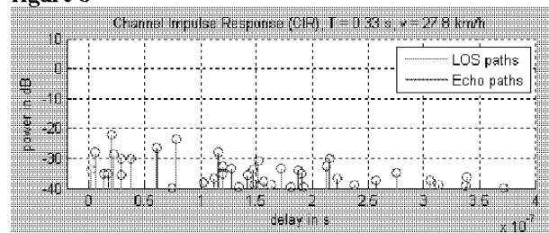
Fig 12: Channel Impulse response corresponding to figure 9
