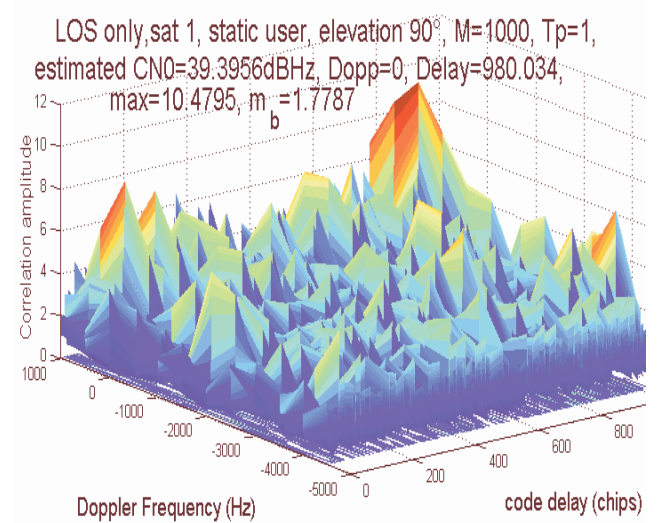
Fig 9: LOS signal of satellite number 1 without multipath replicas or noise, true Doppler 0\text{Hz} , true code delay 608.2758 chips, signal acquired with C/A code of satellite number 11. Estimated values: Doppler frequency 0\text{Hz} , code delay 980.034 chips, C/N_0 39.3956\text{dBHz}
