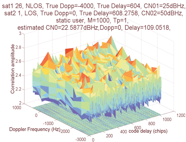
Fig 10: Cross-correlation between 2 GPS signals: 1- Non LOS signal of satellite number 26 (just multipath replicas), true Doppler -4000\text{ Hz} , true delay 604.0\text{ chips} , initial C/N_0\ 25\text{dBHz} 2- LOS signal of satellite number 1 with multipath replicas, true Doppler 0\text{ Hz} , true delay 608.2758\text{ chips} , initial C/N_0\ 50\text{dBHz} . Estimated values: Doppler frequency 0\text{ Hz} , code delay 109.0518\text{ chips} , C/N_0\ 22.5877\text{dBHz}
