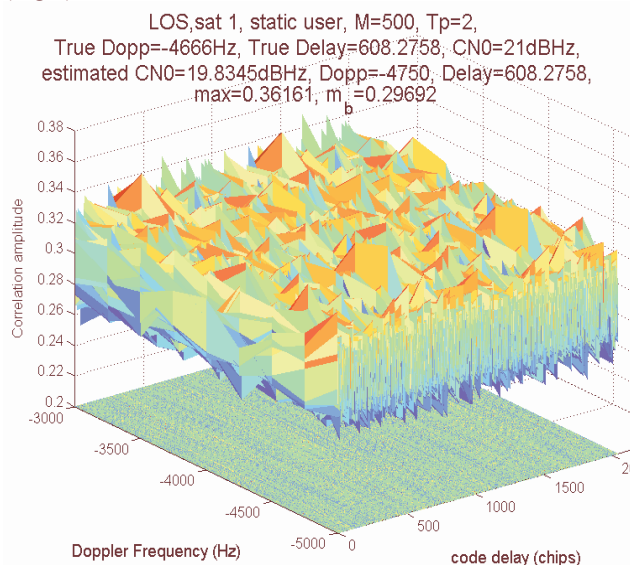
Fig 4: LOS signal with multipath replicas; true values: Doppler frequency -4666\text{Hz} , code delay 608.2758 chips, initial C/N_0 21\text{dBHz} ; estimated values: Doppler frequency -4750\text{Hz} , code delay 608.2758 chips, C/N_0 19.8345\text{dBHz}
