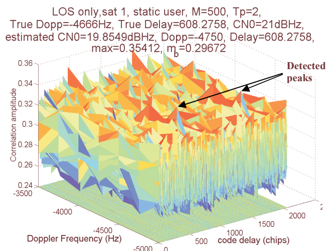
Fig 3: LOS without multipath replicas; true values: Doppler frequency -4666\text{Hz} , code delay 608.2758 chips, initial C/N_0 21\text{dBHz} ; estimated values: Doppler frequency -4750\text{Hz} , code delay 608.2758 chips, C/N_0 19.8549\text{dBHz}
