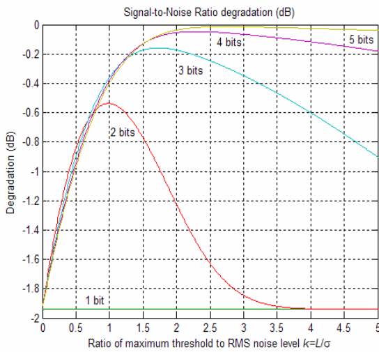
Figure 3 SNR degradation at correlator output due to quantization. Precorrelation filtering and finite sampling frequency effects are neglected
