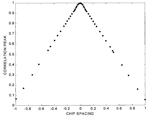
Figure 2.3 Samples sequence for 'peak intensive' distribution
