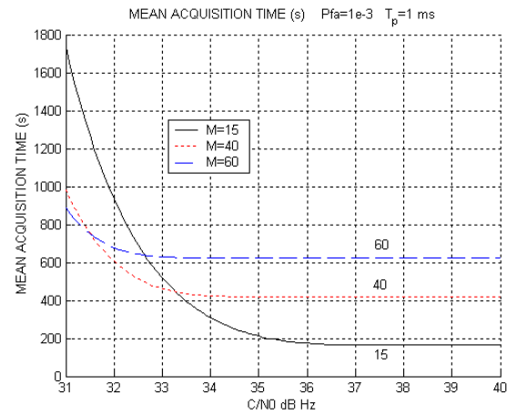
Figure 4: Single dwell search mean acquisition time versus total (I+Q) C/N_0 at antenna output using only one component I or Q for P_{fa} = 1e^{-3} , 1 ms coherent integration time and when searching only one doppler bin and without front end filtering effects
