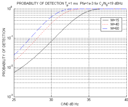
Figure 3: Probability of detection versus total (I+Q) C/N_0 at the antenna output, using only one component I or Q, for 1 ms coherent integration time with the second approach. No uncertainty and no front end filtering effects are assumed
