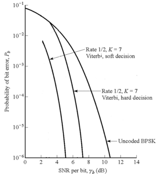
Figure 11: BER for L5 convolutionnal codes using soft and hard Viterbi decoding and BER for uncoded BPSK transmission
