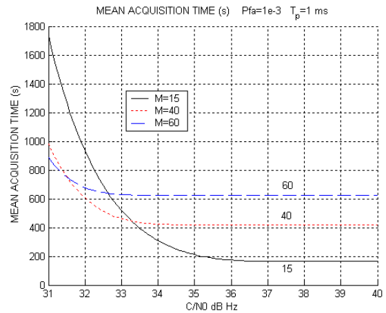
Figure 4: Single dwell search mean acquisition time versus total (I+Q) C/N 0 at antenna output using only one component I or Q for P_{fa}=1e-3 , 1 ms coherent integration time and when searching only one doppler bin and without front end filtering effects
