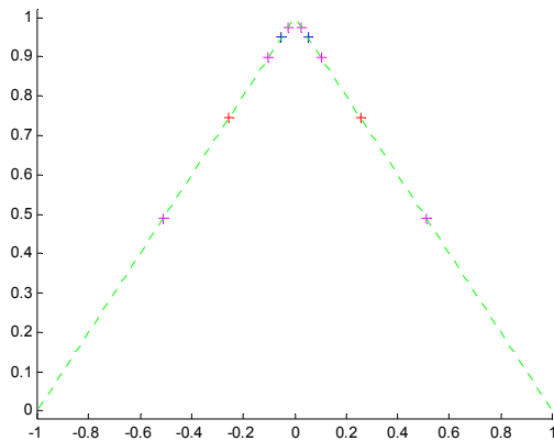
Figure 7: Possible E-L tracking pairs with 3 rd SW version
