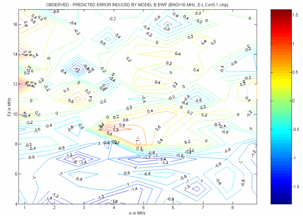
Figure 14: Deviation between the observed and the predicted tracking error (model B evil waveform).
