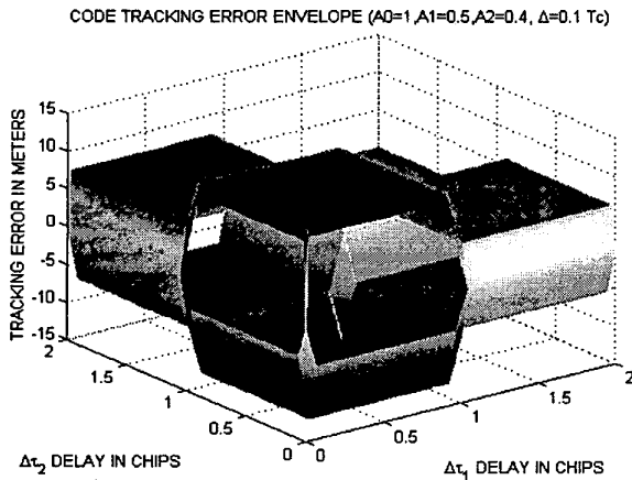
Figure 4: Code tracking error envelope for 2 reflected rays with a total amplitude < LOS amplitude ( 0.1 T_c narrow correlator DLL).
