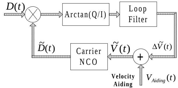
Figure 1-1: Loop with External Velocity Aiding.
