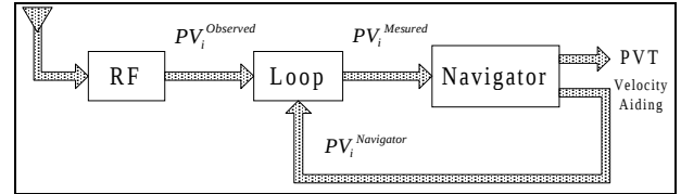
Figure 3-2: Relation between the PseudoVelocity Notations.
