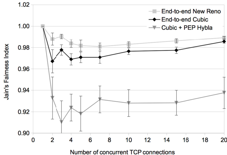
Figure 9. Mean fairness
