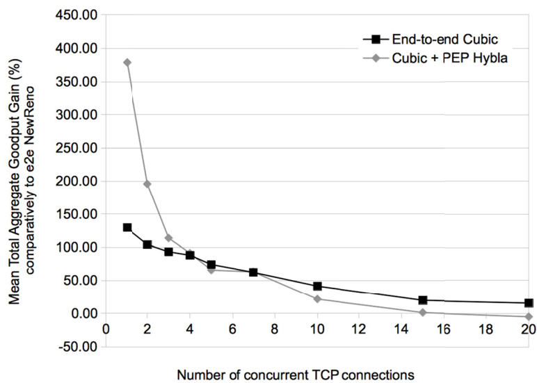
Figure 8. Mean total aggregate goodput gain
