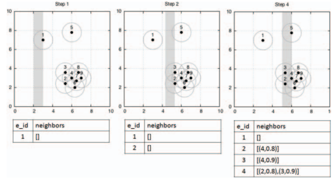
Fig. 9. Illustration of event pre-clustering. The events, represented as two-dimensional points, are ordered according to the x dimension. The neighborhood areas are represented by circles. The lower relevant zone in each step is marked with a gray rectangle.
