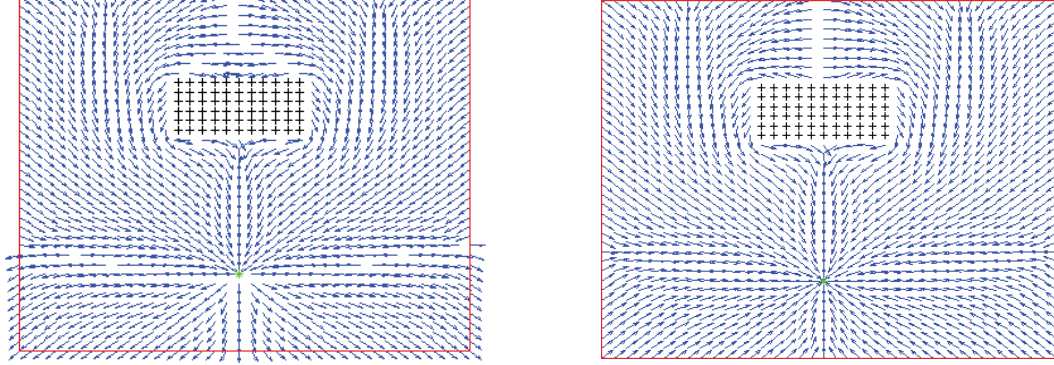
Fig. 1. Biharmonic navigation field, before and after rectification
