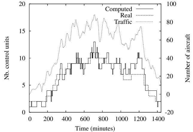
Fig. 5. Number of control sectors (computed schedule, real configurations), and traffic for Brest ATCC (2003, June 1st), with smoothed metrics (SM15)
