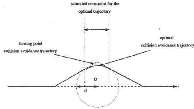
Fig. 1. Comparison optimal trajectory / turning point
