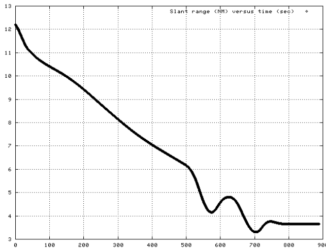
Figure 6: Actual slant range (in NM) between the two aircraft as a function of time (in sec)
