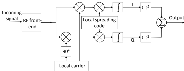
Fig. 7: Correlation process scheme
