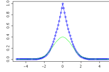
Figure 5. The maximum specified possibility distribution for N(0,1) .
