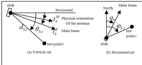
Figure 2. Horizontal and vertical angles
