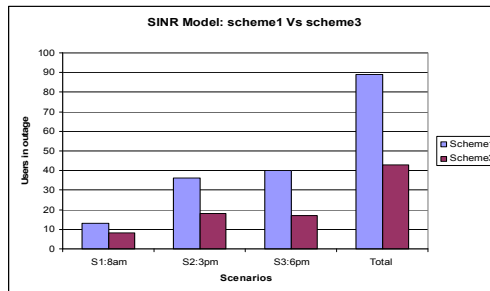
Figure 5. Reuse scheme 1 and scheme 3 results with 3 scenarios
