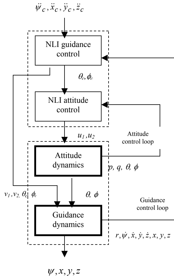
Figure 2-Proposed control structure
