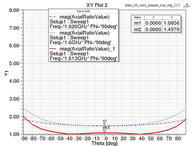
Figure 9: Antenna axial ratio at the minimal (blue dashed curve), central (continue red curve), and maximal (magenta dashed curve) frequencies of the bandwidth
