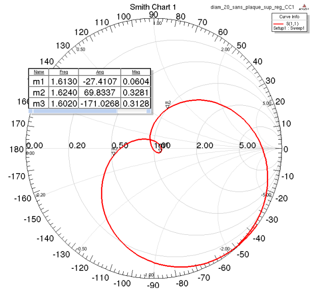
Figure 8: Smith chart of the antenna reflection coefficient ( S_{11} )
