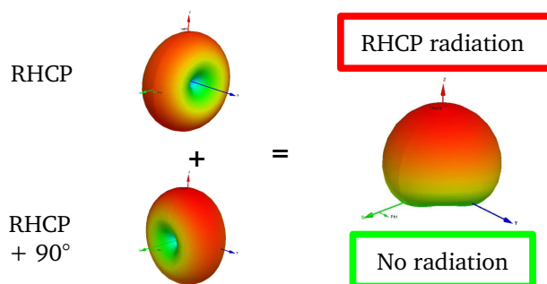
Figure 3: Half-directional radiation pattern
