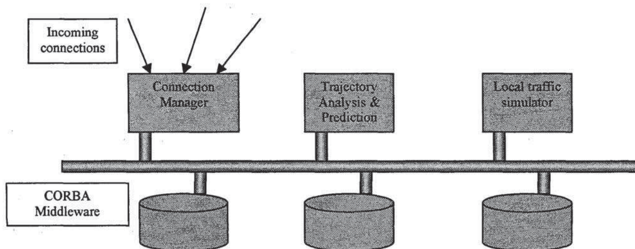
Figure 3. Services Communication
