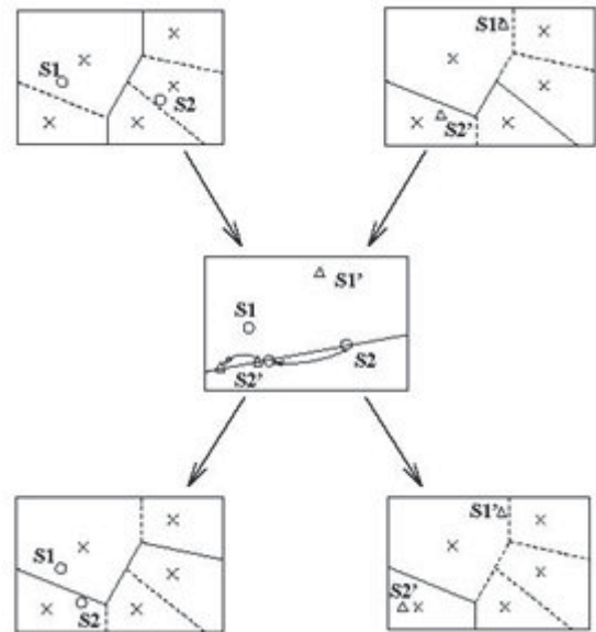
Figure 11. Crossover Operator
