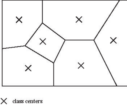
Figure 3. Random Sectoring by Voronoi Diagram
