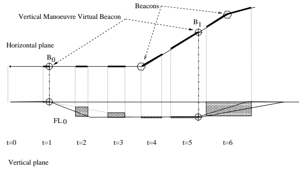
Figure 7: Vertical maneuver during the cruising period.
