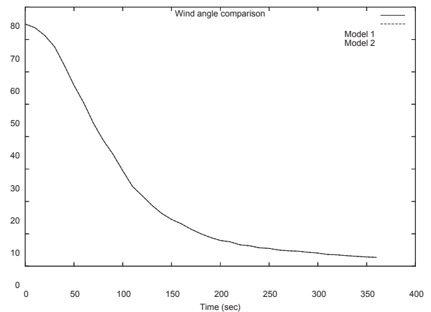
Figure 7. Wind Angle Convergence Phase for the Model 1 and 2
